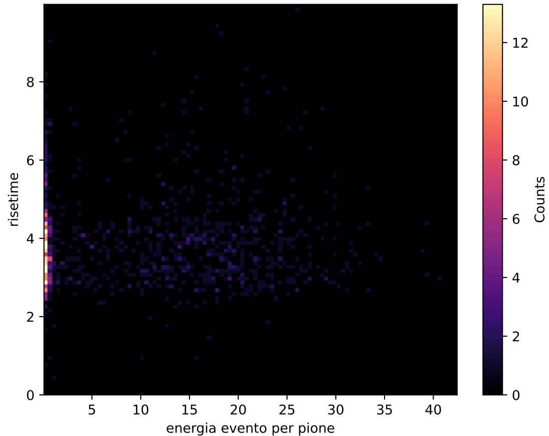
pion distribution 40.0GeV
