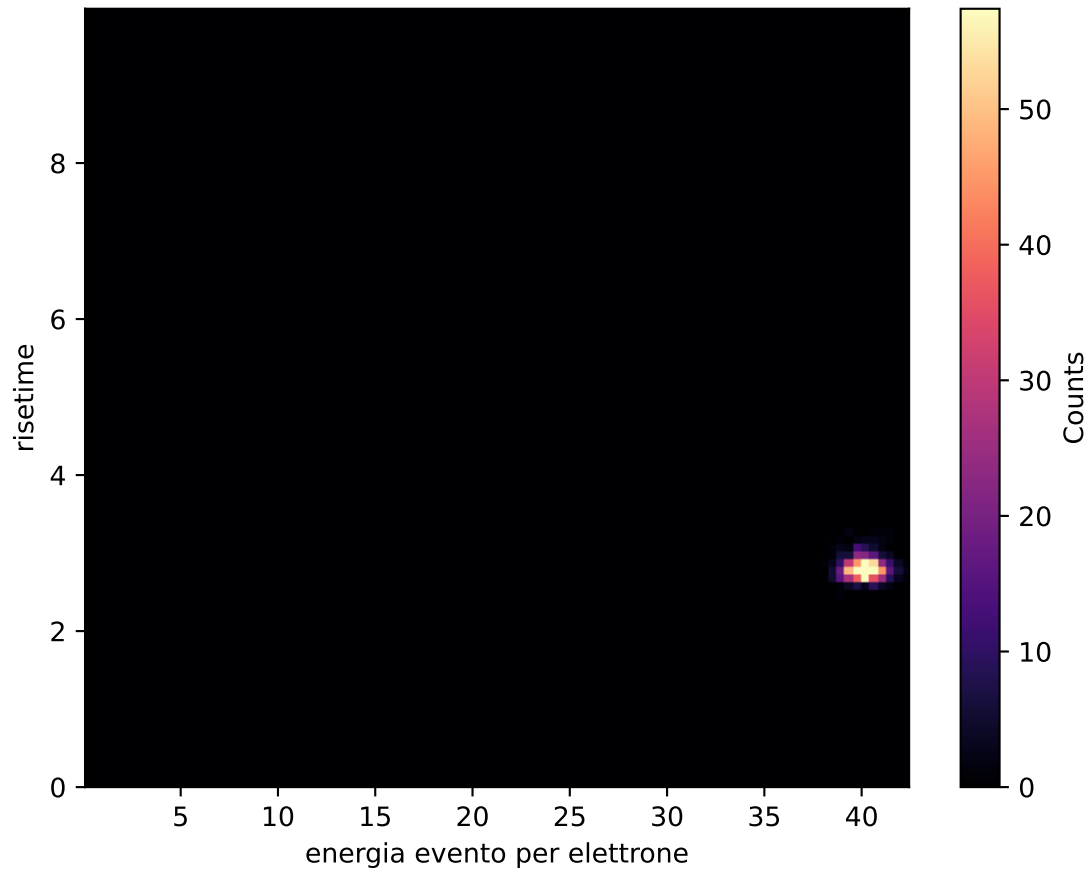
electron distribution 40.0GeV
